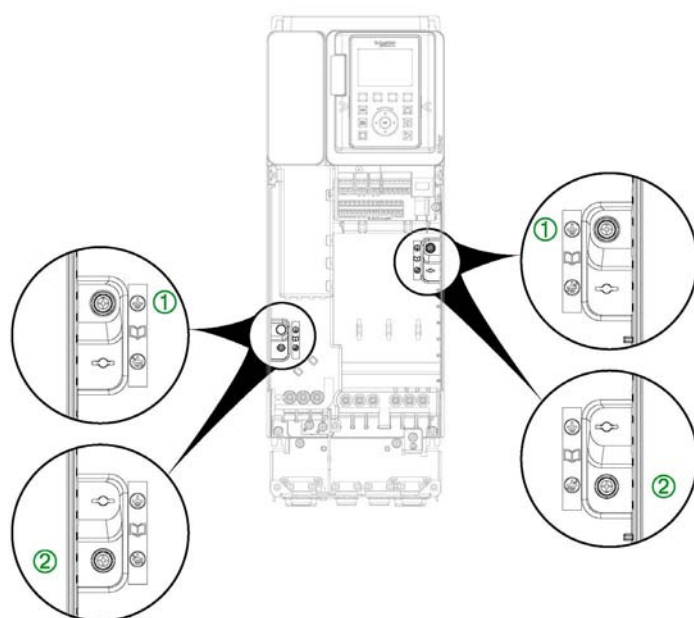
Setting For Frame Size 2, Frame Size 3 and IP55 Frame Size A Products
